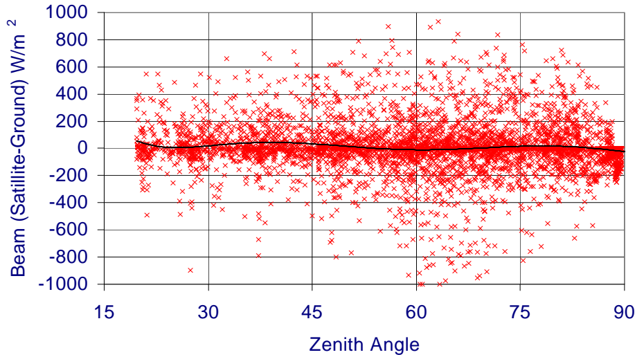
Fig. 6: Plot of the difference between ground-based and satellite-derived beam irradiance versus zenith angle. The trend line shows there is little or no systematic deviation about the zenith angle.
