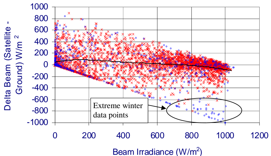
Fig. 3: Difference between hourly beam irradiance obtained from satellite modeling and ground-based measurements. Small blue circles are December, January, and February data points. The red X's are data from the rest of the year.
