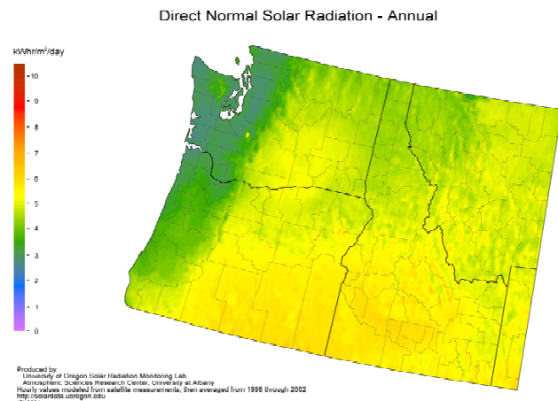
Fig. 1: Annual Pacific Northwest direct normal irradiance from satellite derived solar radiation database.
